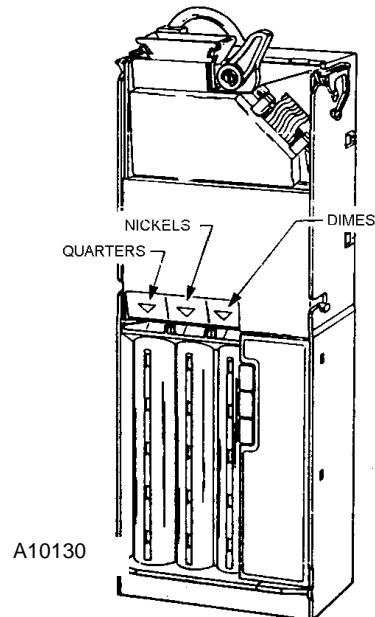
FIGURE 4. Coin Tubes
