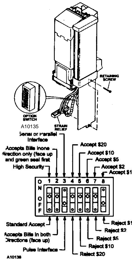
FIGURE 10. Validator Option Switches
