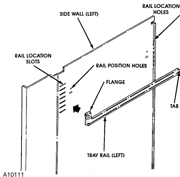
FIGURE 15. Tray Rail
