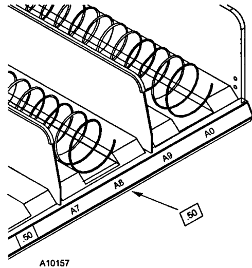
Figure 19. Price Labels
