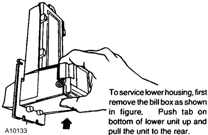
FIGURE 13. Remove Lower Housing
