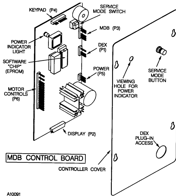
FIGURE 8. Control Board
