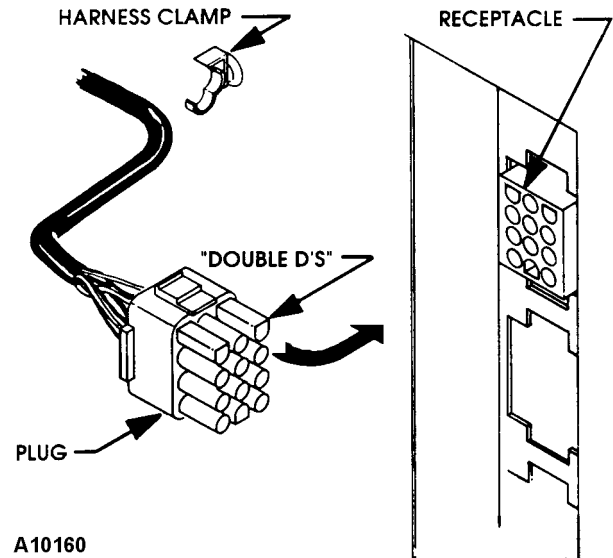
FIGURE 14. Tray Harness
