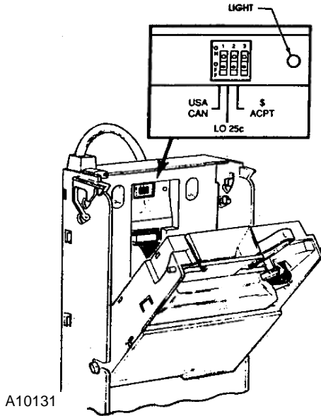
FIGURE 5. Option switches
