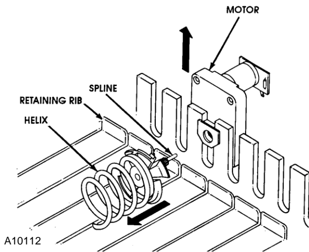
FIGURE 17. Helix Coupling
