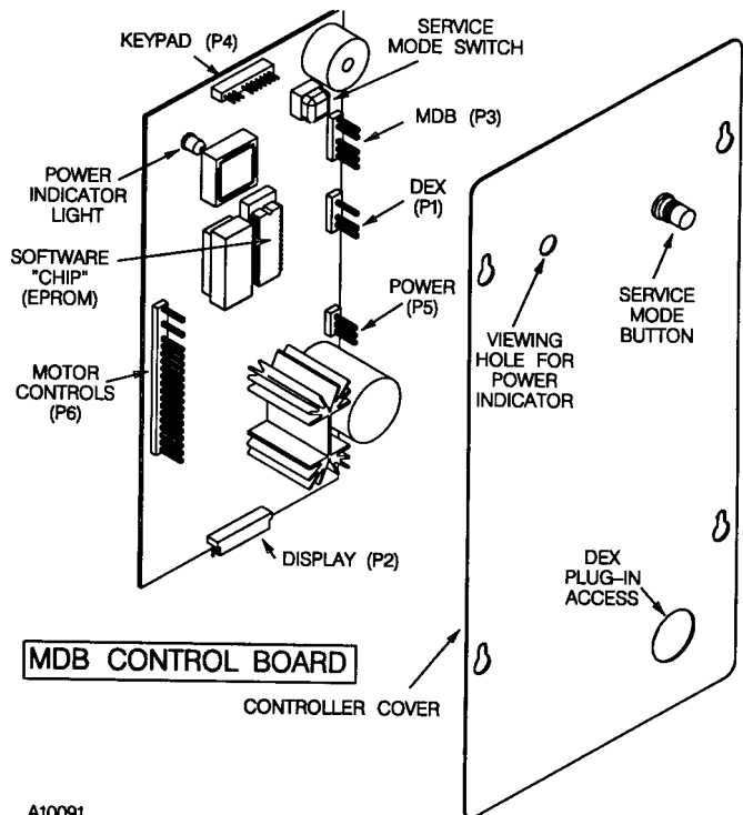
FIGURE 7. Control Board
